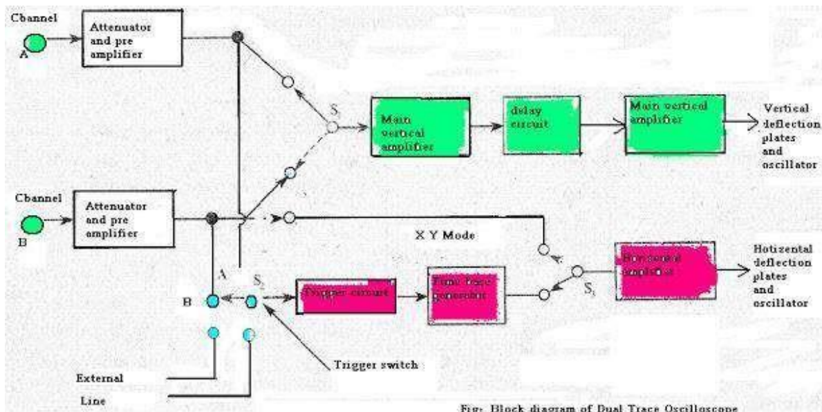
Fig: Block diagram of Dual Trace Oscilloscope
