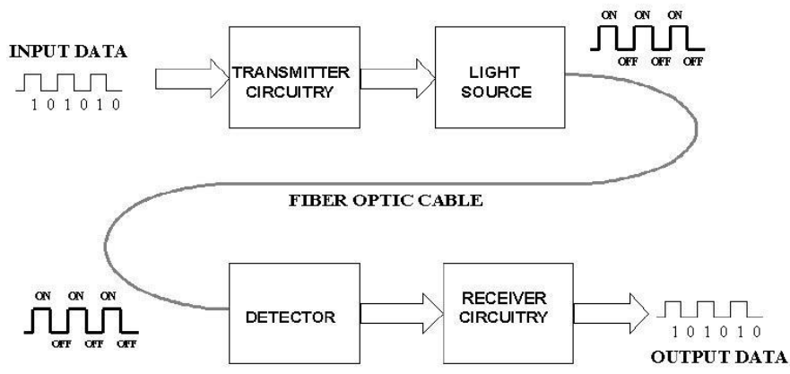
Working of Fiber optic communication
